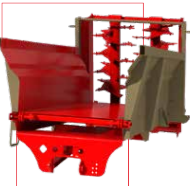
Monoblock, tapered body with one-piece side sheets for easy unloading of the goods.
