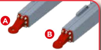
Choice of eyelets (A) Bolted Ø 50 mm (standard) (B) Bolted knee-joint (option)
